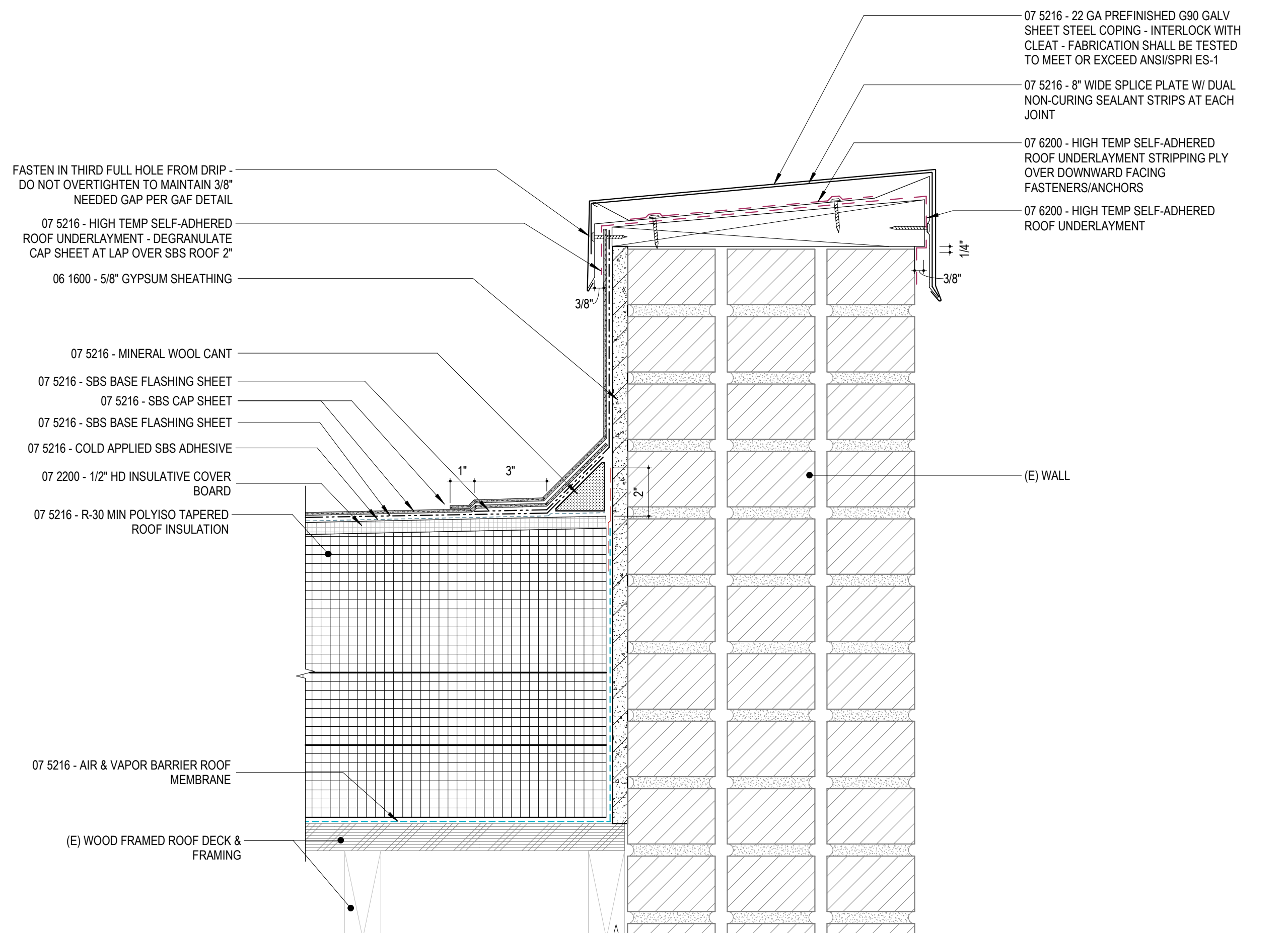
2-PLY SBS MEMBRANE - PARAPET W/ NEW COPING AT (E) MASONRY WALL ② 3" = 1'-0"
