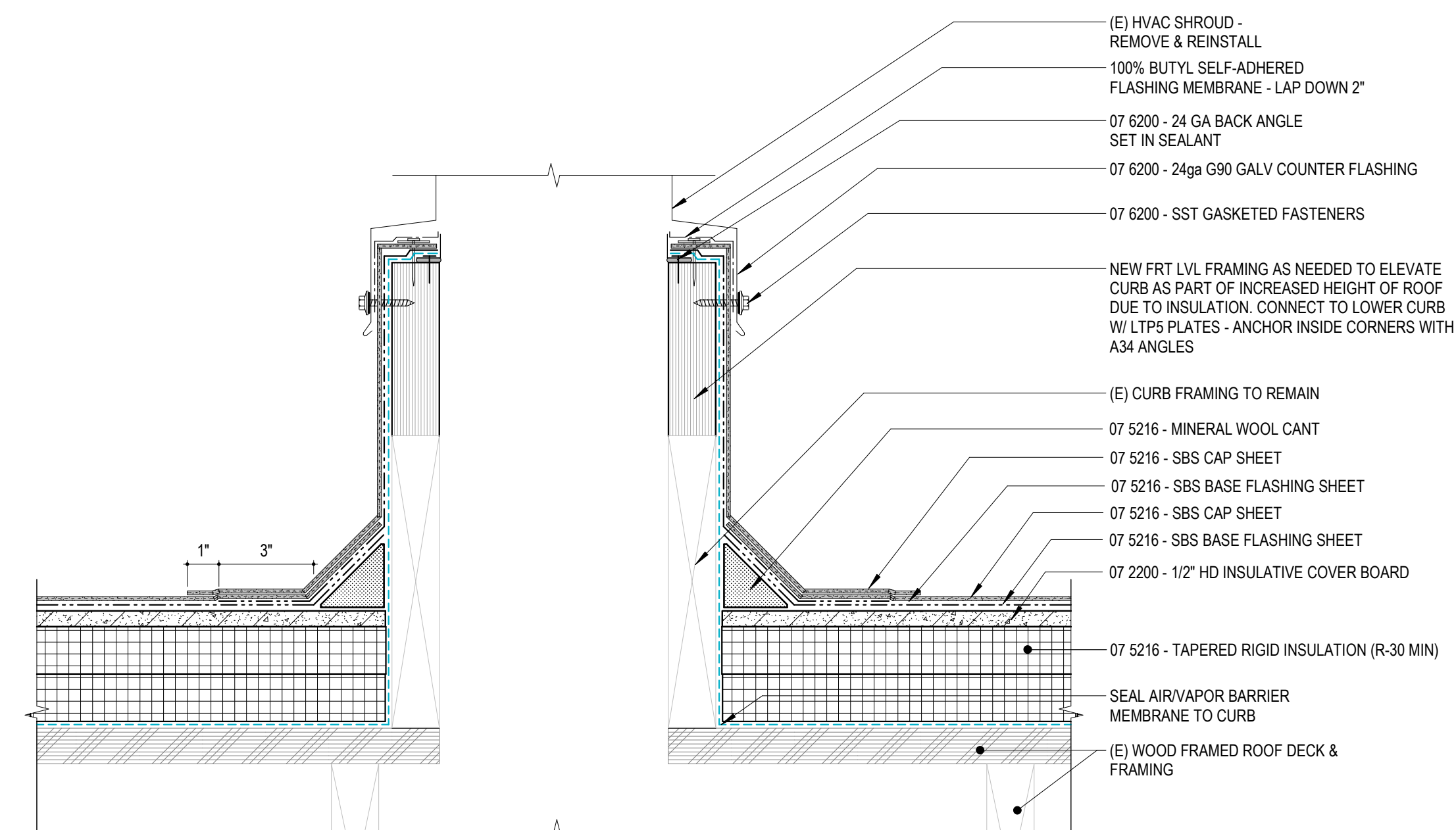
2-PLY SBS MEMBRANE - TYPICAL MECH CURB - WOOD ⑤ 3" = 1'-0"
