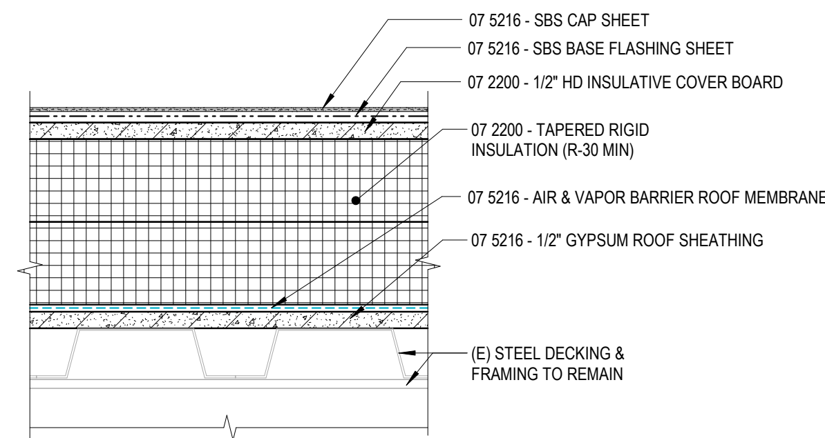
2-PLY SBS MEMBRANE - TYPICAL ROOF ASSEMBLY - STEEL DECK ①
