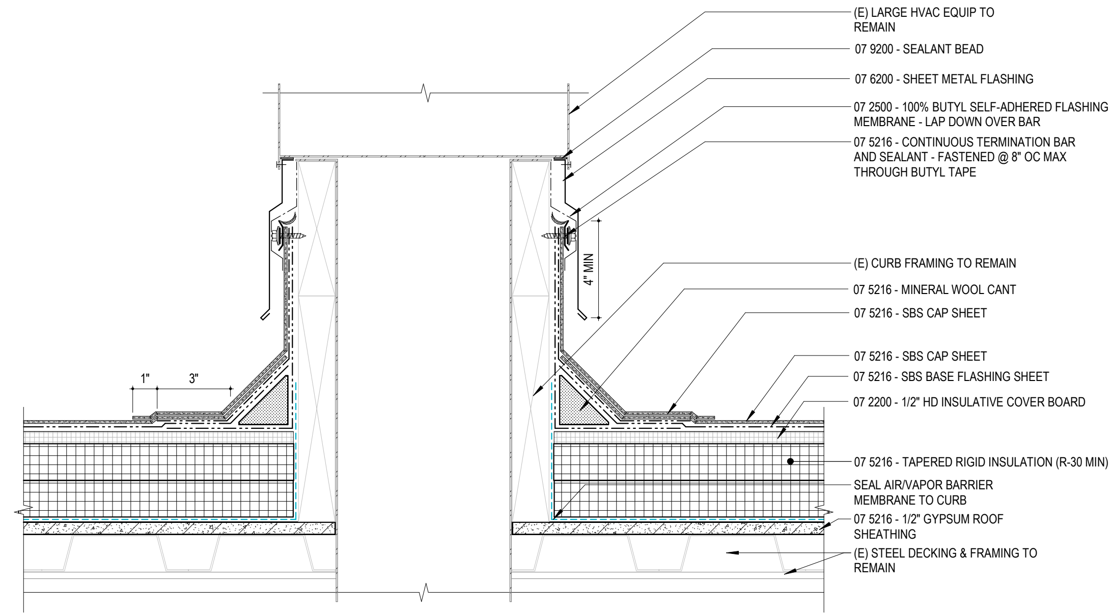
2-PLY SBS MEMBRANE - LARGE MECH EQUIP CURB - STEEL ⑥
