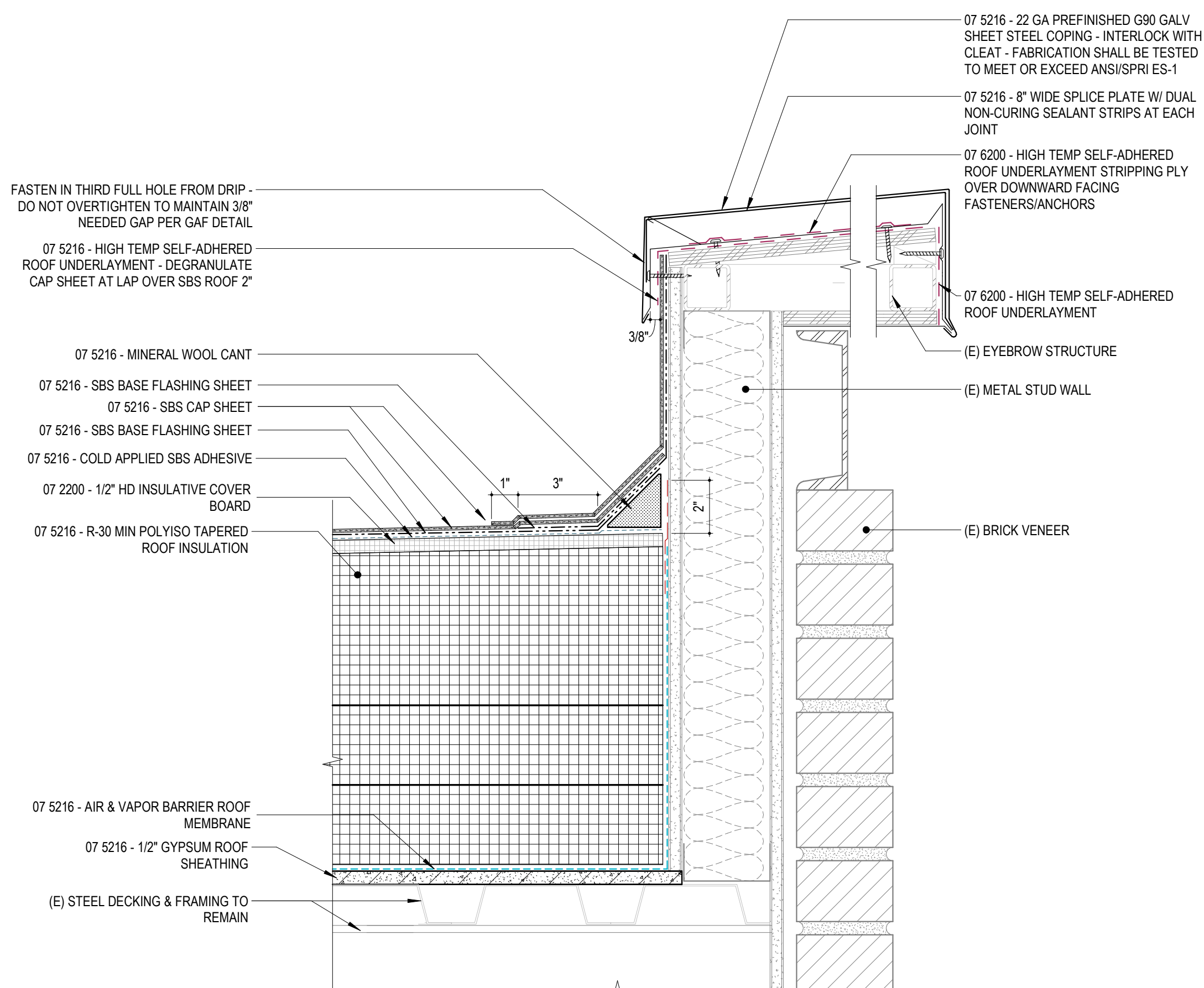
2-PLY SBS MEMBRANE - PARAPET W/ NEW COPING AT (E) METAL STUD WALL AND STEEL DECK ③
