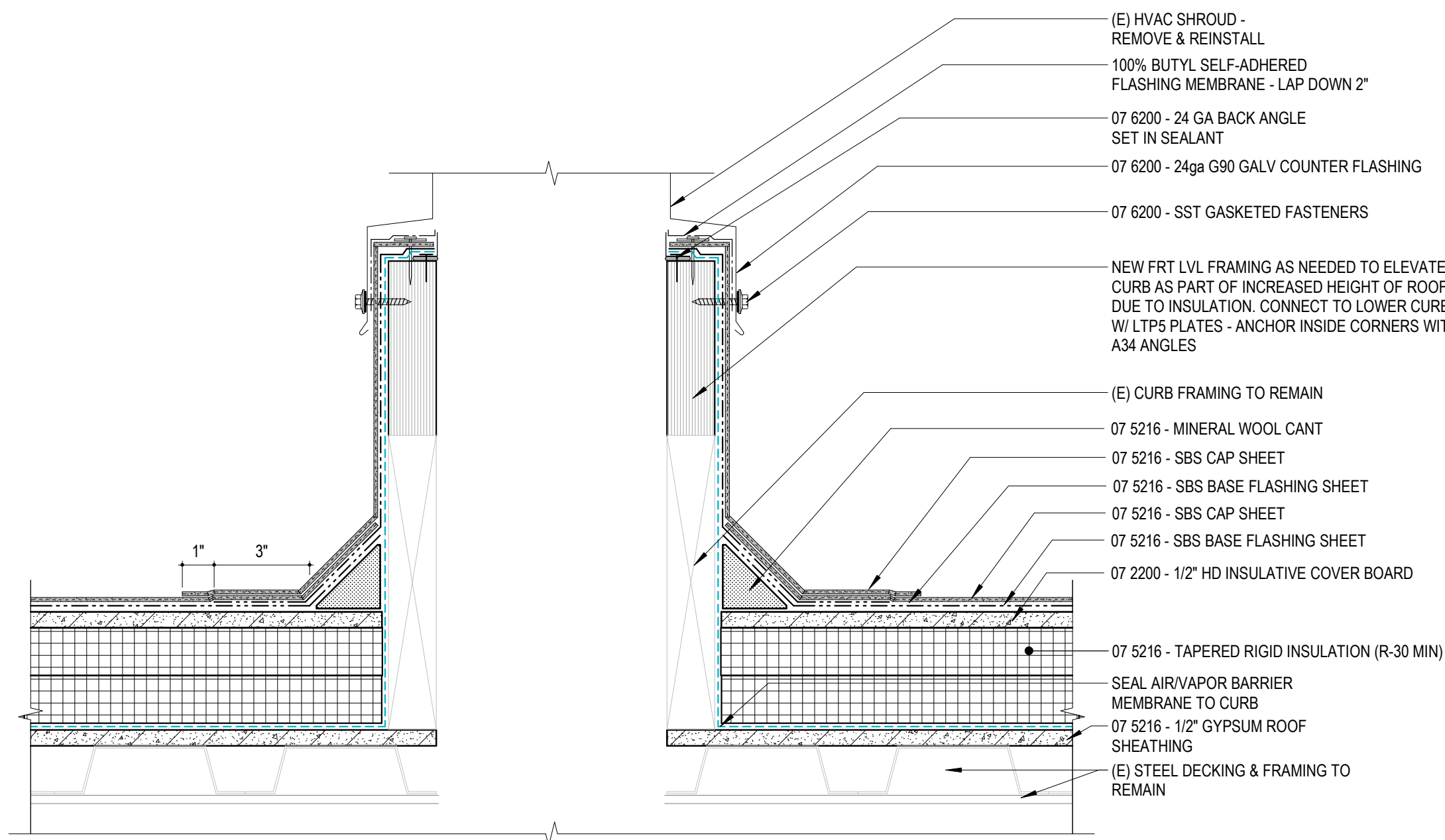
2-PLY SBS MEMBRANE - TYPICAL MECH CURB - STEEL ⑤
