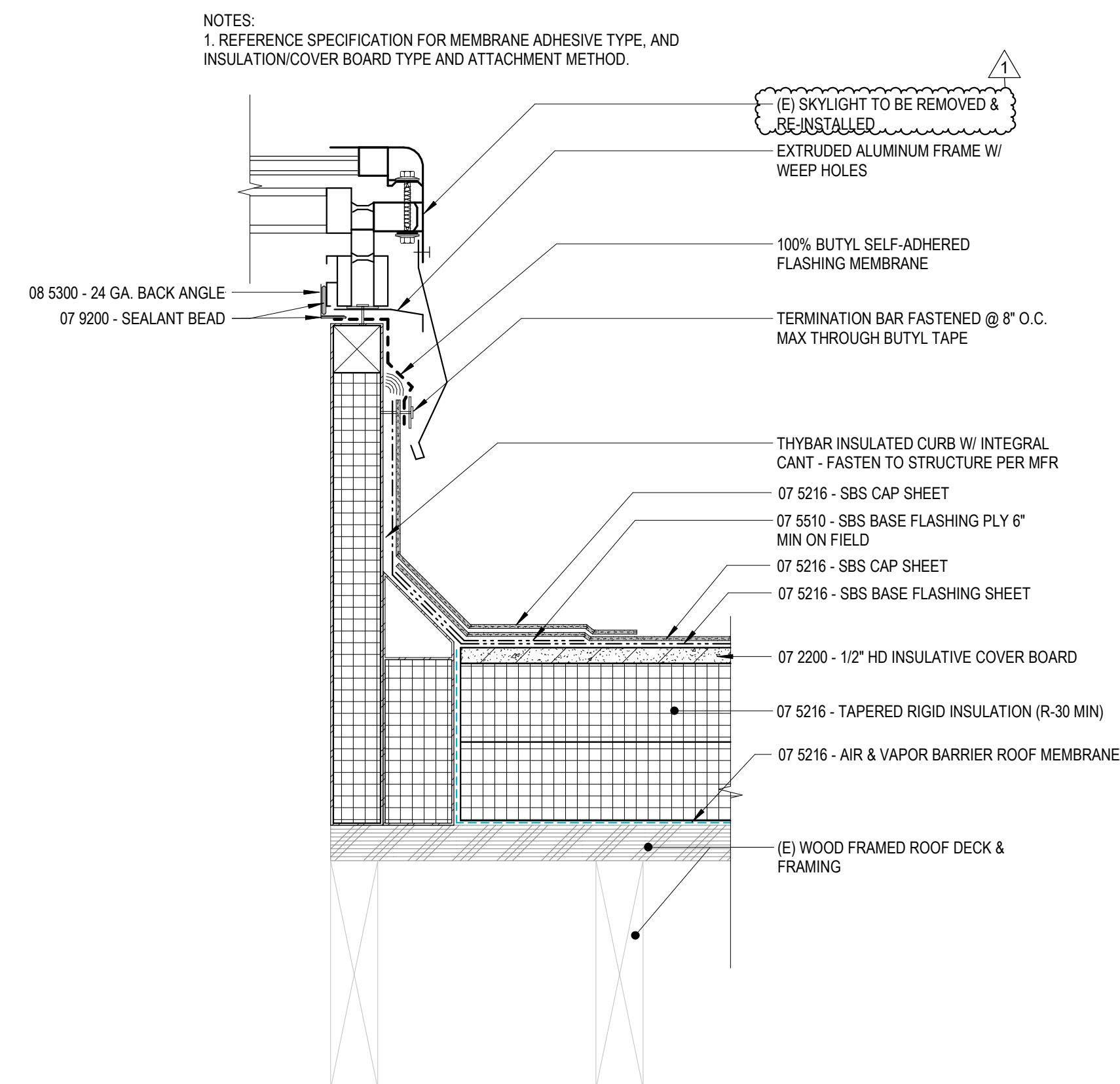
2-PLY SBS MEMBRANE - TYPICAL ROOF HATCH/SKYLIGHT - WOOD ③ 3" = 1'-0"
