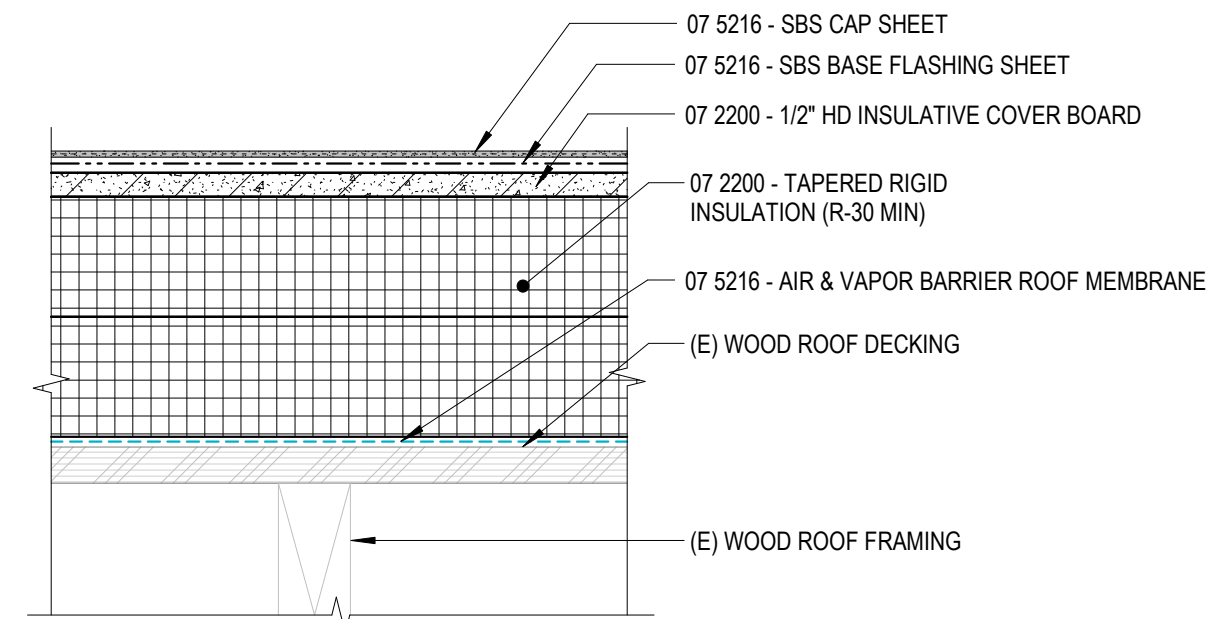
2-PLY SBS MEMBRANE - TYPICAL ROOF ASSEMBLY - WOOD ① 3" = 1'-0"
