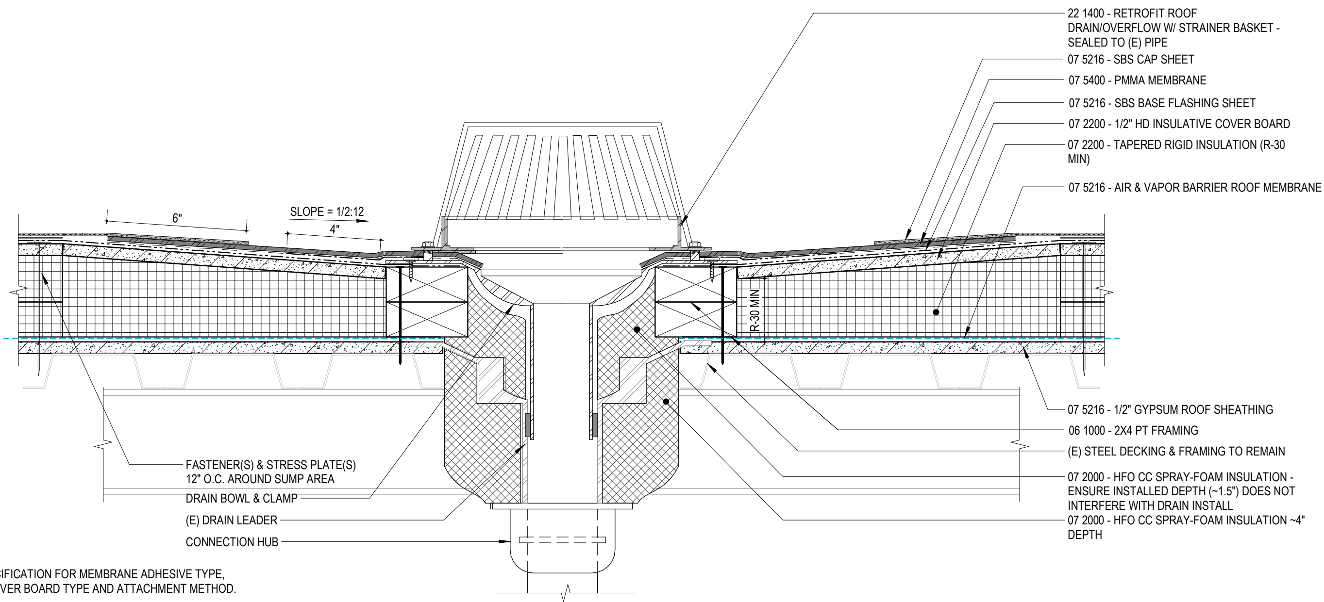
2-PLY SBS MEMBRANE - ROOF DRAIN - STEEL ④
