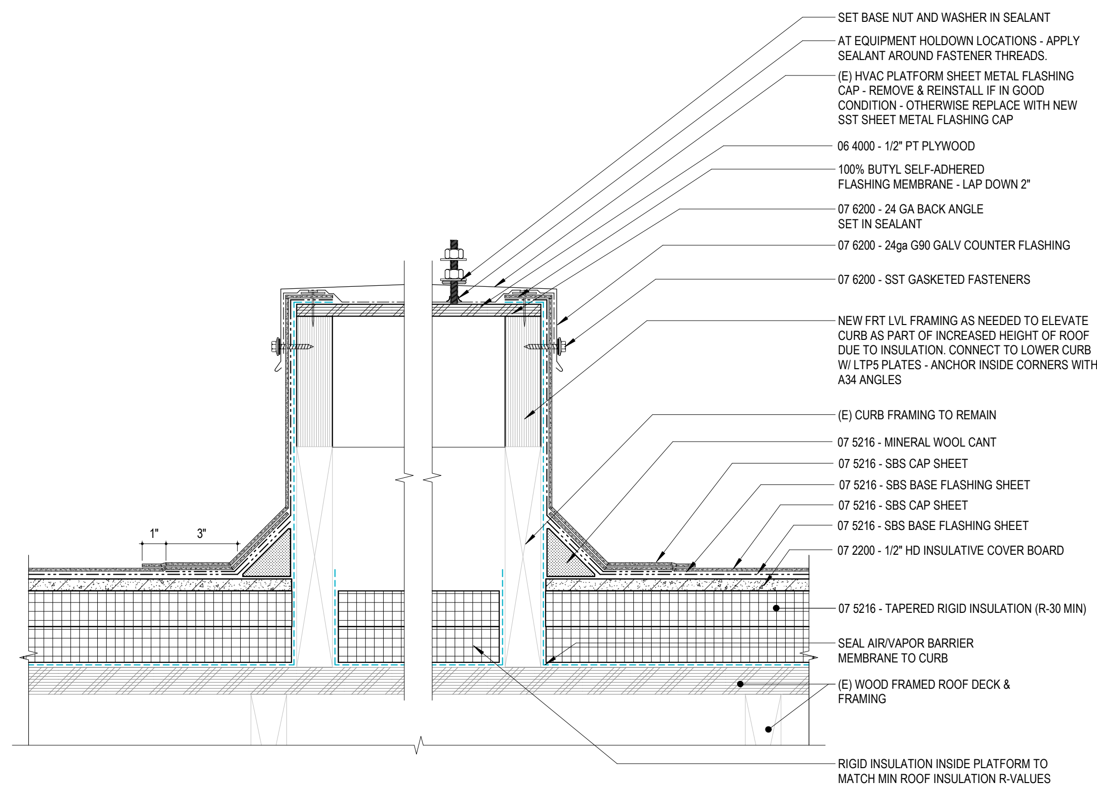
2-PLY SBS MEMBRANE - TYPICAL MECH CURB - WOOD ⑧ 3" = 1'-0"
