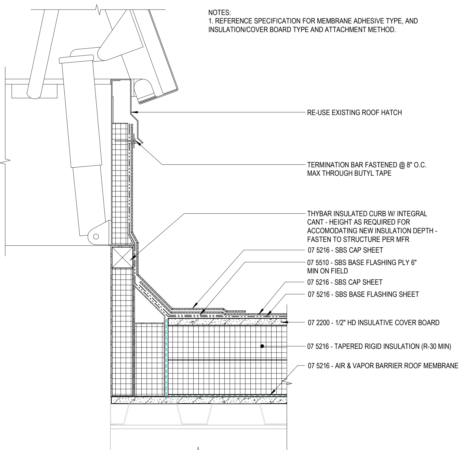
2-PLY SBS MEMBRANE - TYPICAL ROOF HATCH/SKYLIGHT - WOOD ⑧
