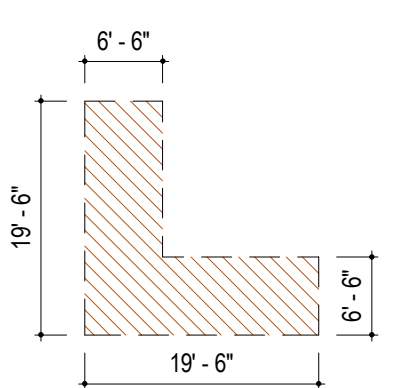
TYPICAL ZONE 3 DIAGRAM N.T.S.
