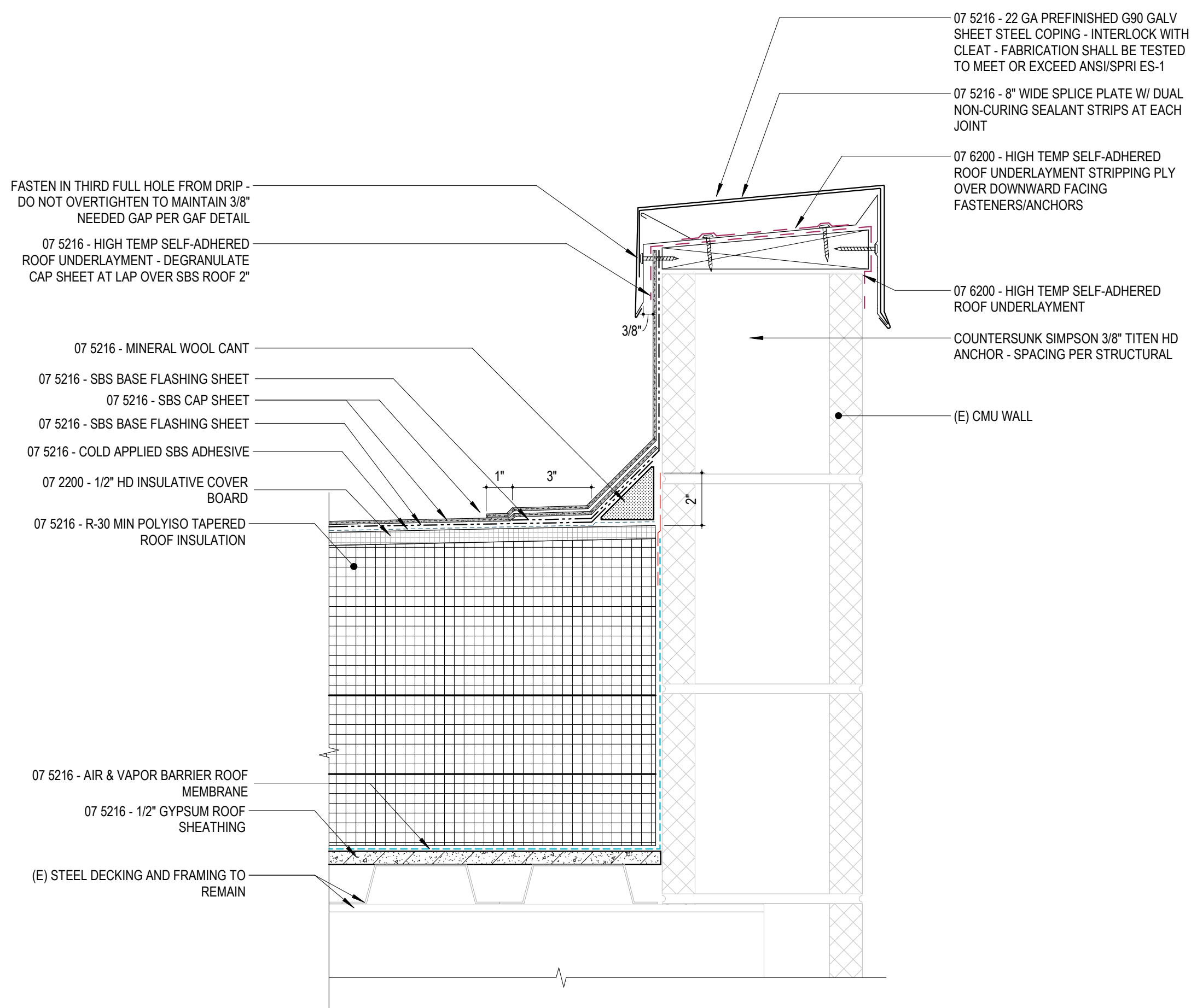
2-PLY SBS MEMBRANE - PARAPET W/ NEW COPING AT (E) CMU WALL AND STEEL DECK ②
