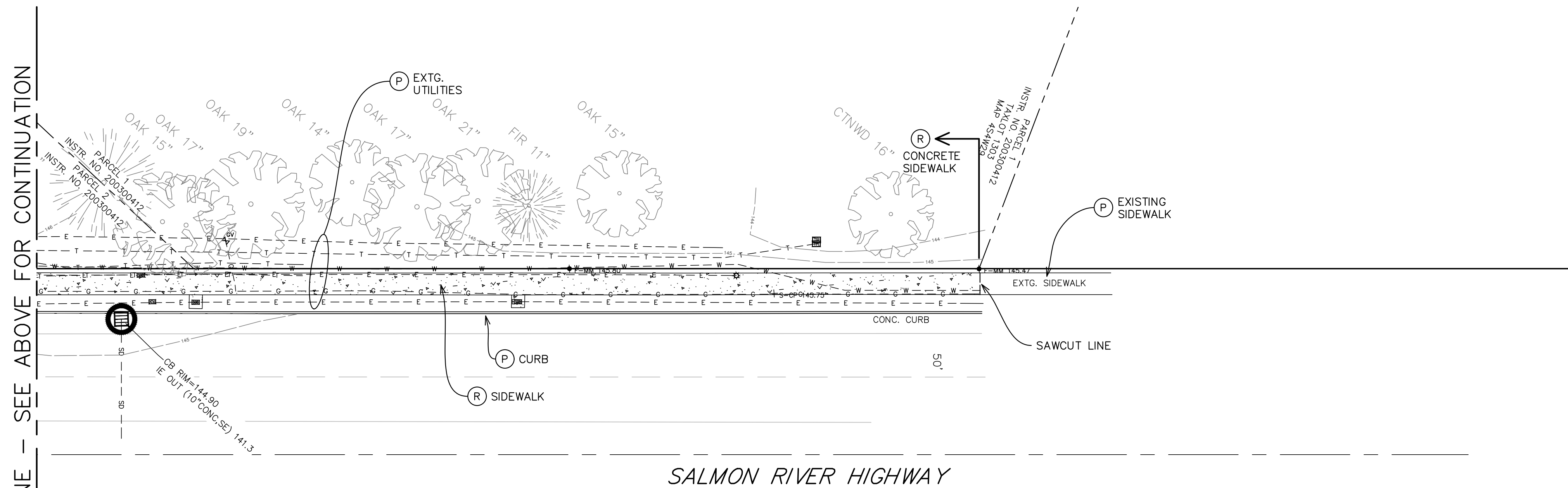
SALMON RIVER HIGHWAY EXISTING CONDITIONS/ EROSION CONTROL/ DEMOLITION PLAN
