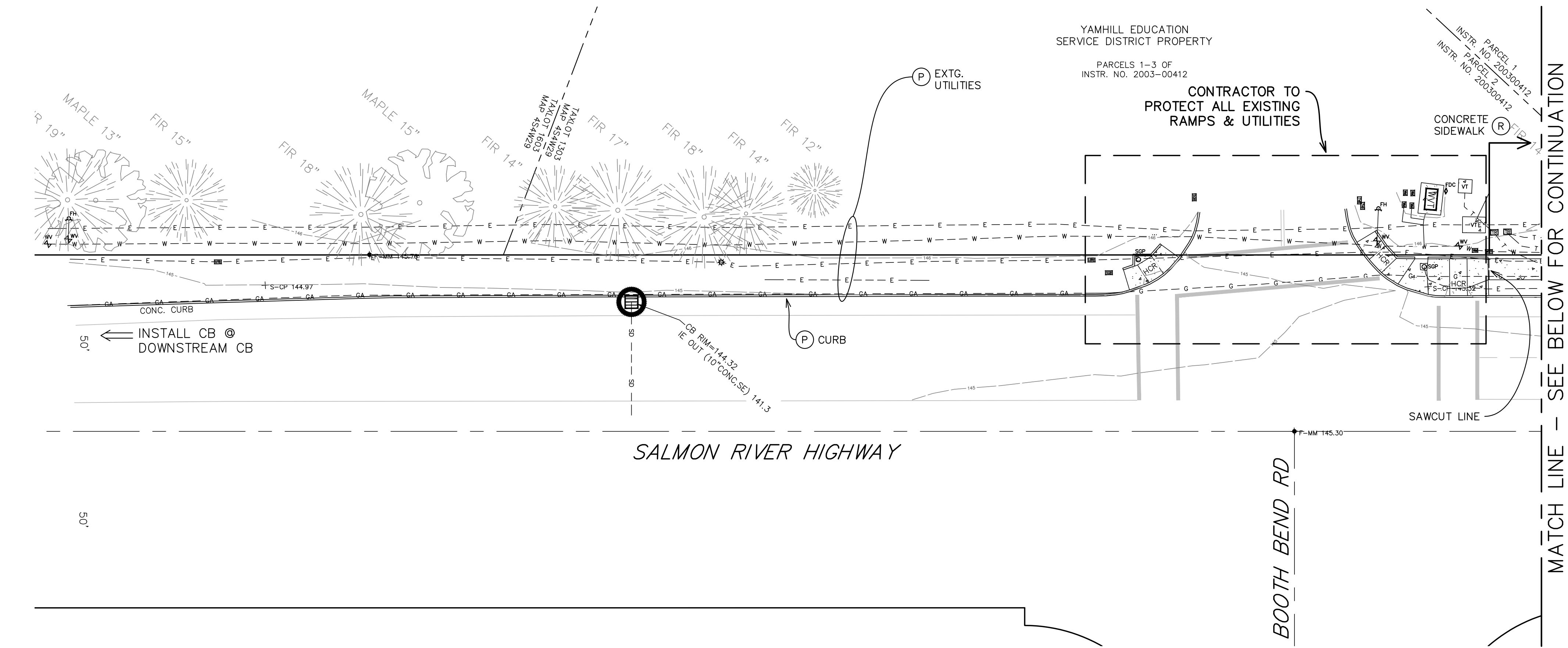
SALMON RIVER HIGHWAY EXISTING CONDITIONS/ EROSION CONTROL/ DEMOLITION PLAN
