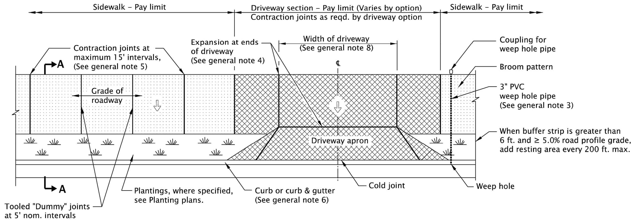
TYPICAL PLAN VIEW - SEPARATED SIDEWALK
