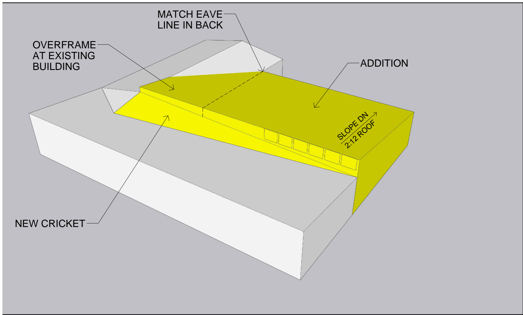
C1 CONCEPTUAL FRAMING AXONOMETRIC SCALE: 1/4" = 1'-0"
