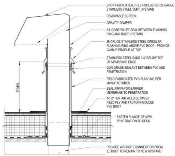
HVAC DUCT PENETRATION
