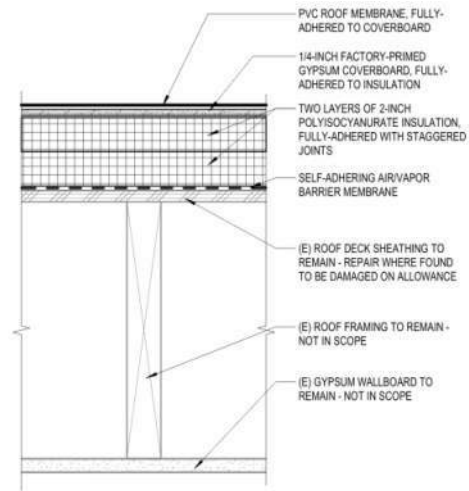
LOW SLOPE ROOF ASSEMBLY
