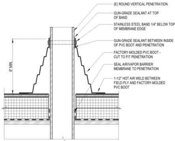
PLUMBING STACK PENETRATION
