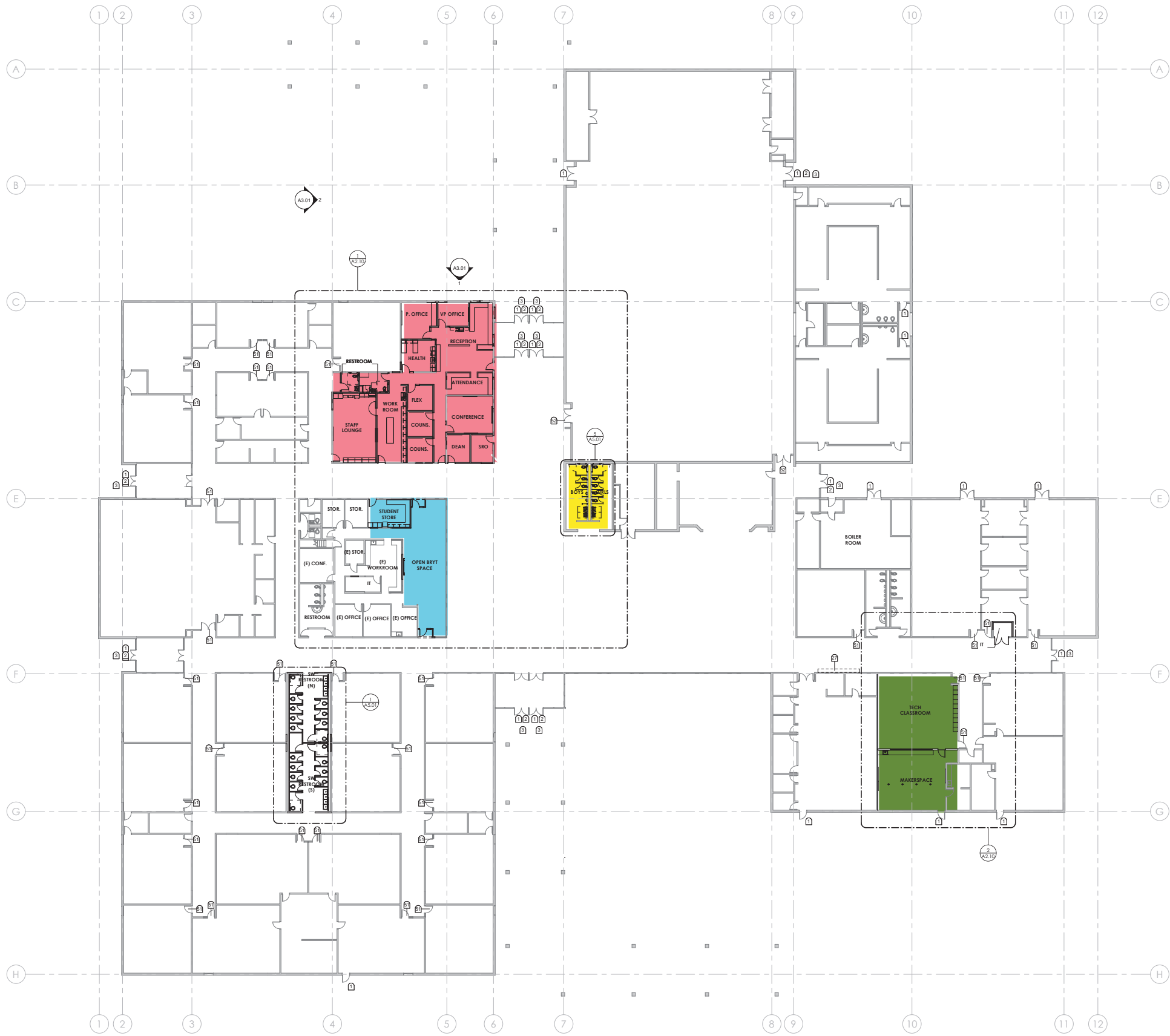
1 OVERALL FLOOR PLAN - LEVEL 1 V2.01 SCALE: 1/16" = 1'-0"
